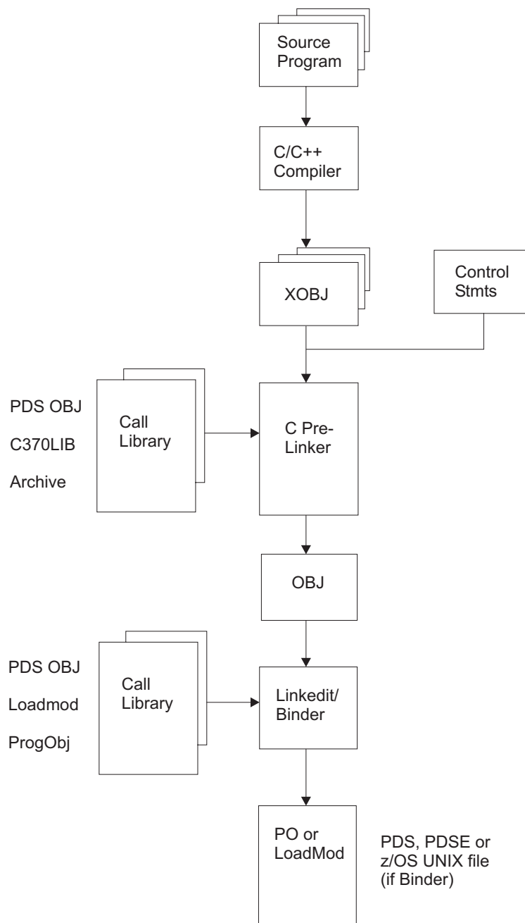
Figure 44. Invoking the prelinker. This diagram shows where the prelinker is invoked when the binder 'prelinker' function is not used.
