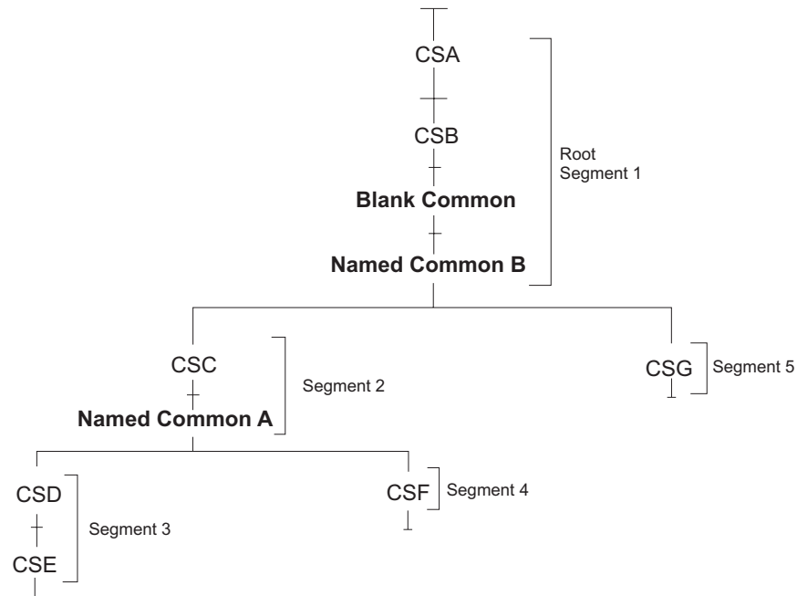
Figure 58. Common areas after processing
