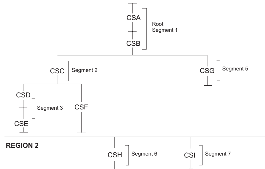
Figure 54. Overlay tree for multiple-region program
