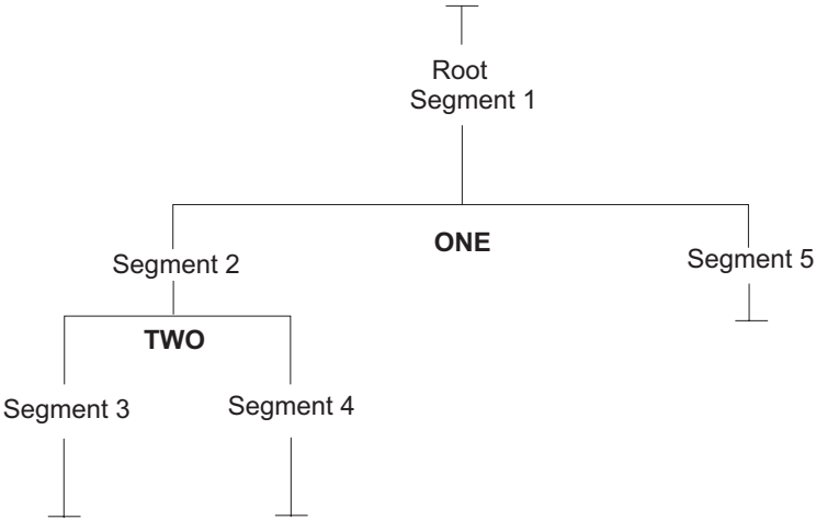
Figure 55. Symbolic segment origin in single-region program
