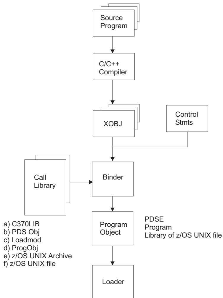
Figure 45. Prelinker elimination. This is the optional control flow in the z/OS binder.
