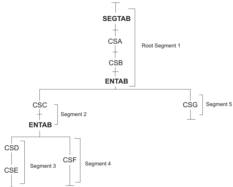
Figure 52. Location of segment and entry tables in an overlay module
