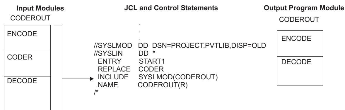
Figure 16. Deleting a section
