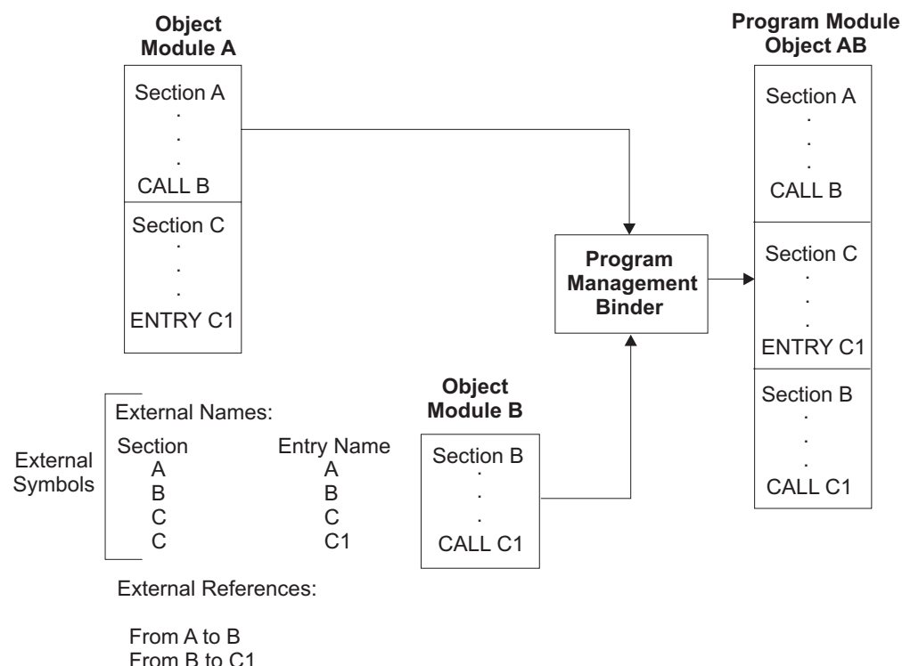
Figure 4. External names and external references
