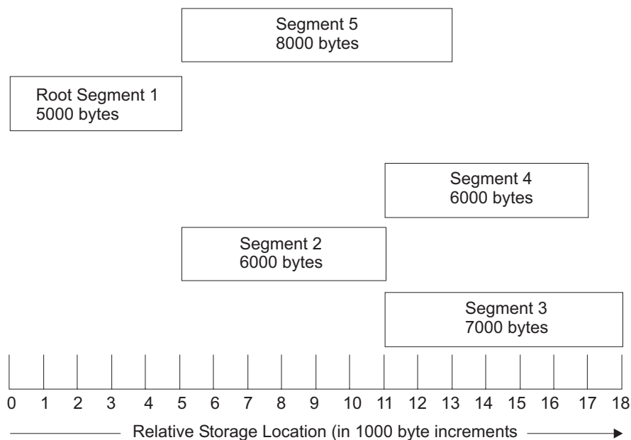
Figure 49. Segment origin and use of storage
