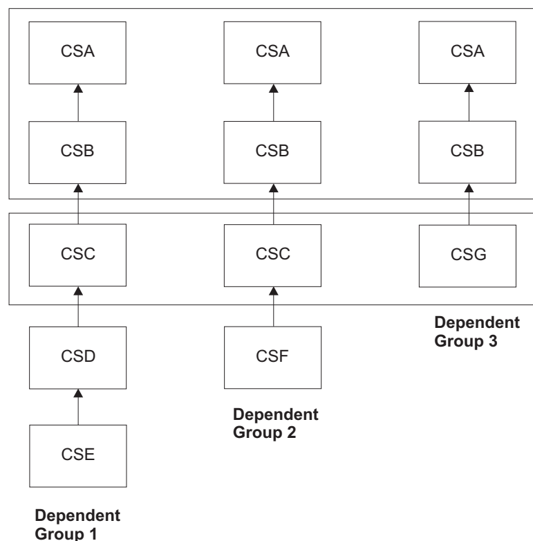
Figure 46. Control section dependencies
