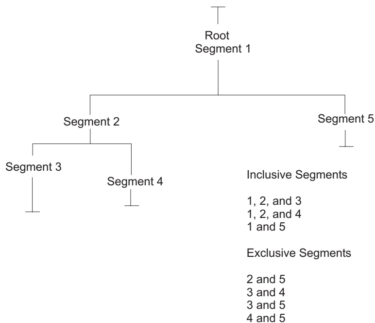
Figure 50. Inclusive and exclusive segments
