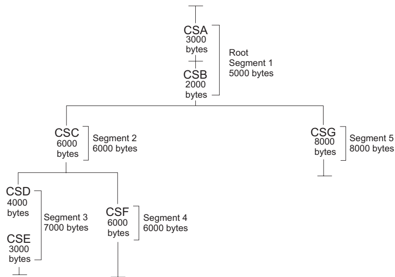
Figure 48. Length of an overlay module
