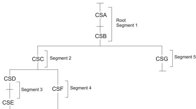
Figure 47. Single-region overlay tree structure
