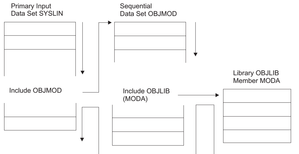
Figure 11. Processing of nested INCLUDE control statements
