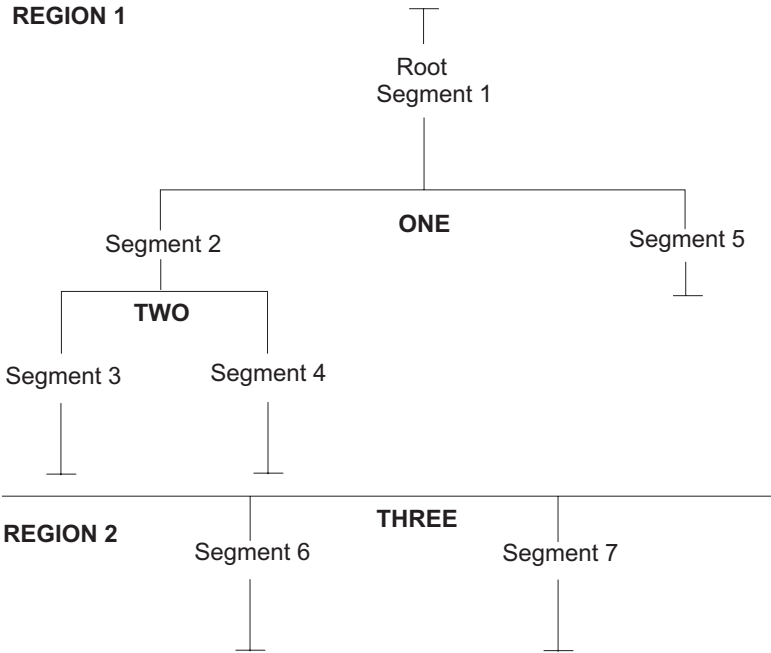
Figure 56. Symbolic segment and region origin in multiple-region program
