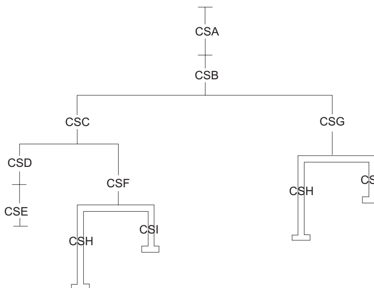
Figure 53. Control sections used by several paths
