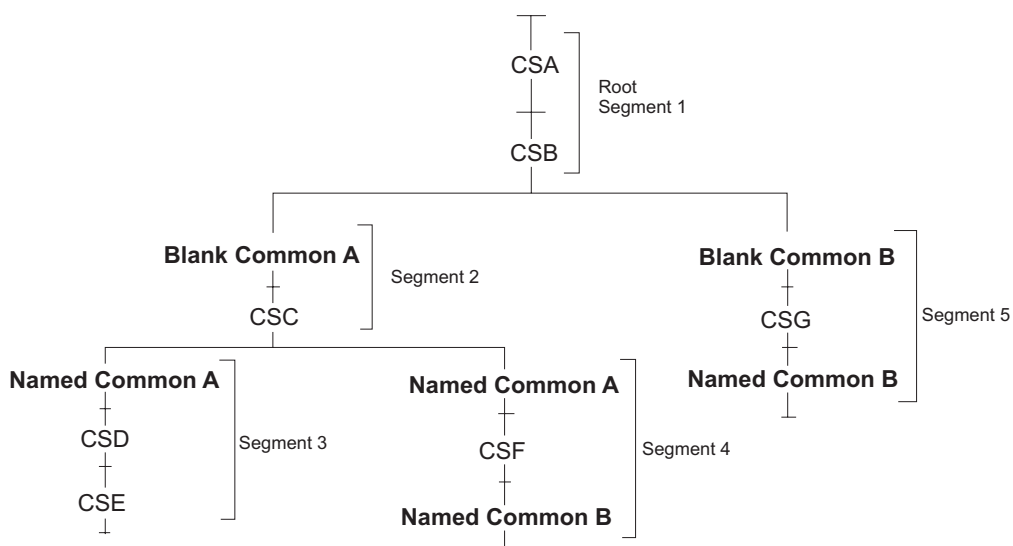
Figure 57. Common areas before processing
